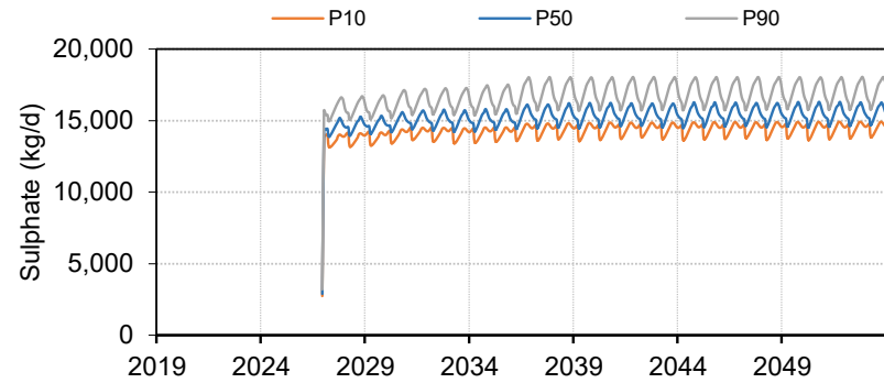
(b) Sulphate Load Reduction (kg/d)
