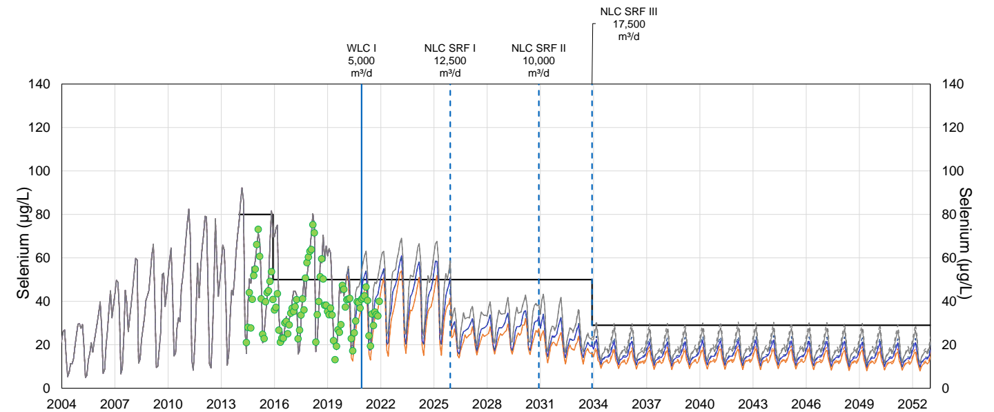
Figure C-5: Projected Concentrations of Nitrate, Selenium, and Sulphate at the LCO Compliance Point (LC_LCDSSLCC; E297110) with West Line Creek Groundwater Water Availability Decreased from 60% to 50%
