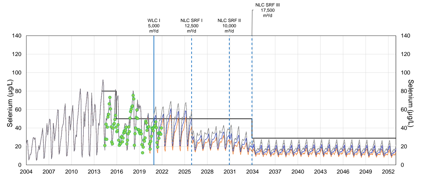
Figure C-6: Projected Concentrations of Nitrate, Selenium, and Sulphate at the LCO Compliance Point (LC_LCDSSLCC; E297110) with West Line Creek Groundwater Water Availability Increased from 60% to 70%
