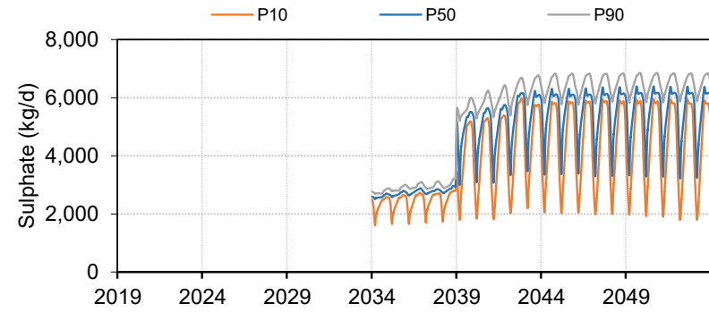
(b) Sulphate Load Reduction (kg/d)
