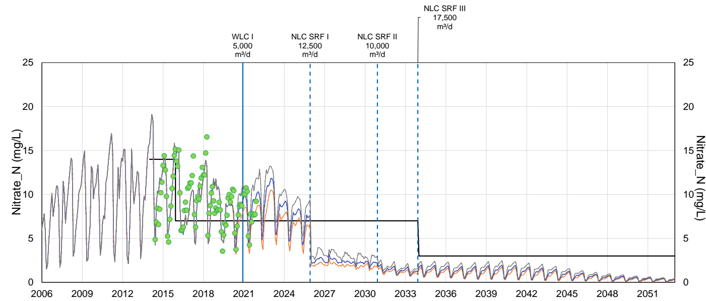
Figure C-6: Projected Concentrations of Nitrate, Selenium, and Sulphate at the LCO Compliance Point (LC_LCDSSLCC; E297110) with West Line Creek Groundwater Water Availability Increased from 60% to 70%
