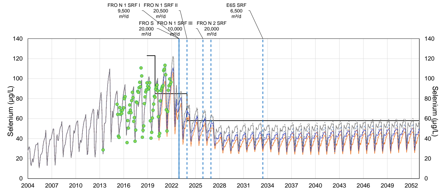
Figure C-4: Projected Concentrations of Nitrate, Selenium, and Sulphate at the FRO Compliance Point (FR_FRABCH; E223753) with Clode Creek Water Availability Decreased from 85% to 60%
