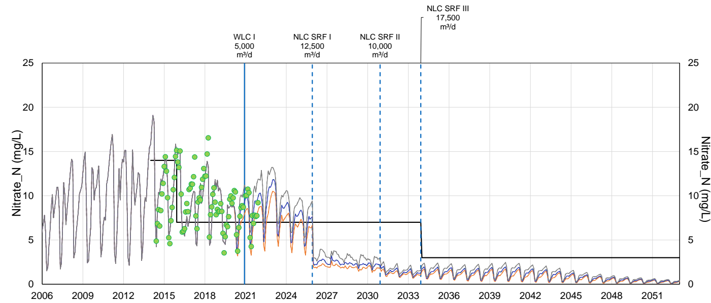
Figure C-5: Projected Concentrations of Nitrate, Selenium, and Sulphate at the LCO Compliance Point (LC_LCDSSLCC; E297110) with West Line Creek Groundwater Water Availability Decreased from 60% to 50%
