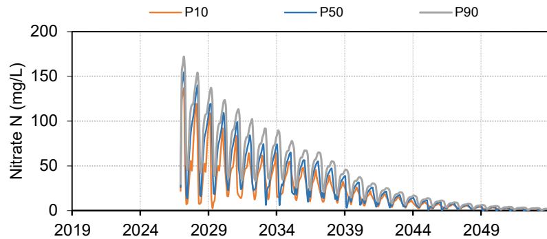
(c) Nitrate Influent Concentration (mg/L)
