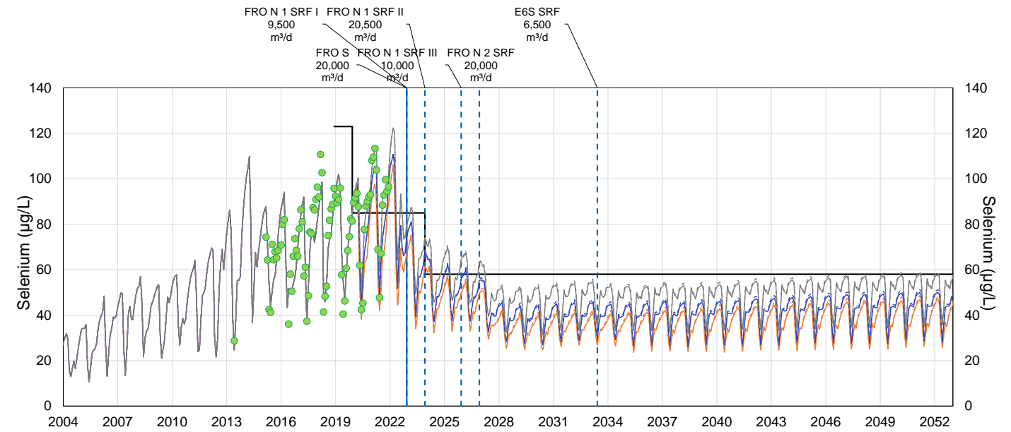
Figure C-3: Projected Concentrations of Nitrate, Selenium, and Sulphate at the FRO Compliance Point (FR_FRABCH; E223753) with Clode Creek Water Availability Decreased from 85% to 75%
